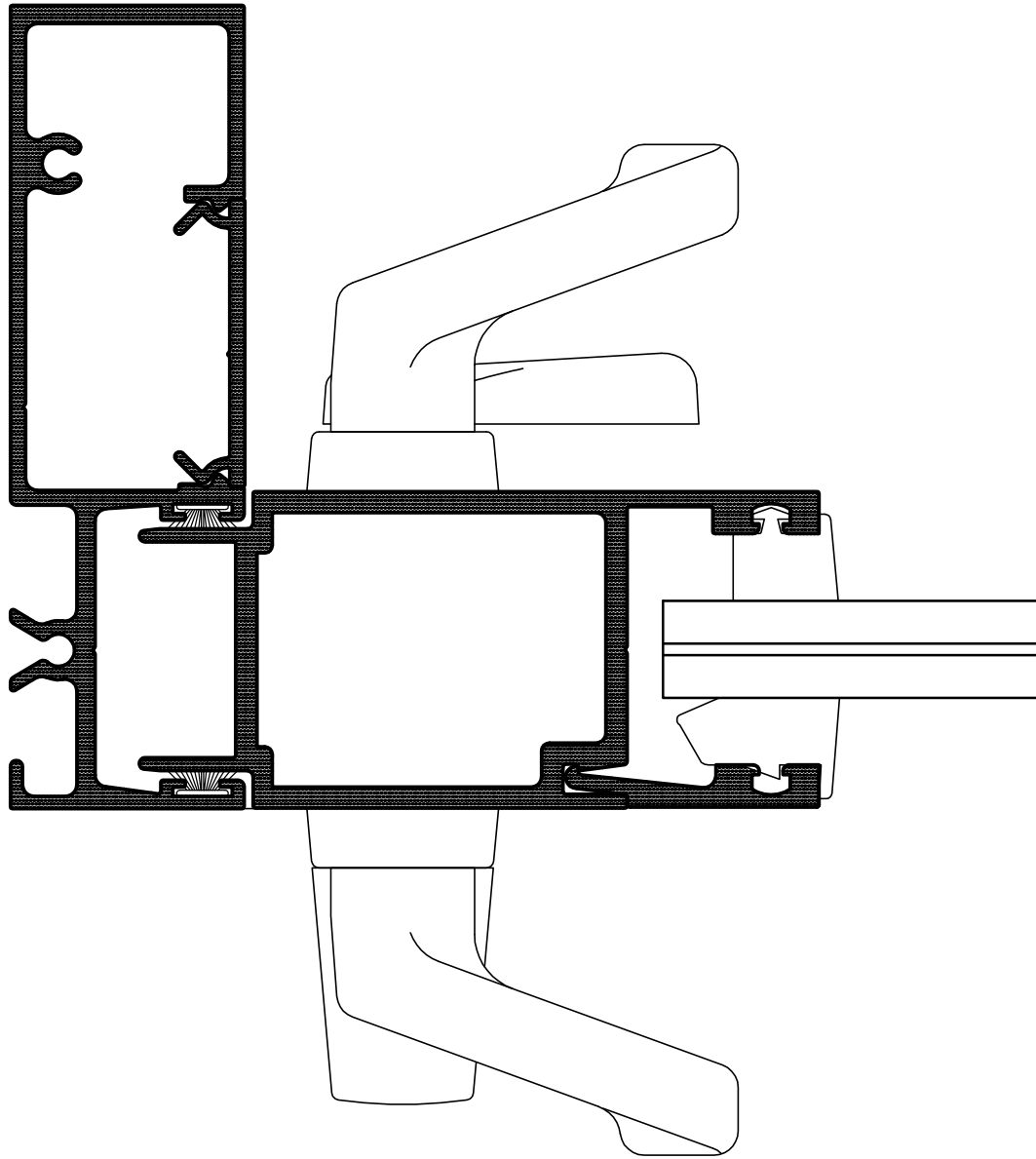
3 MOVING PANEL JAMB
